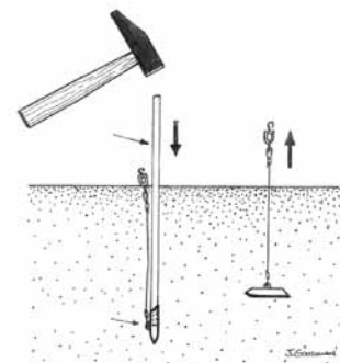
Earth Anchor.
