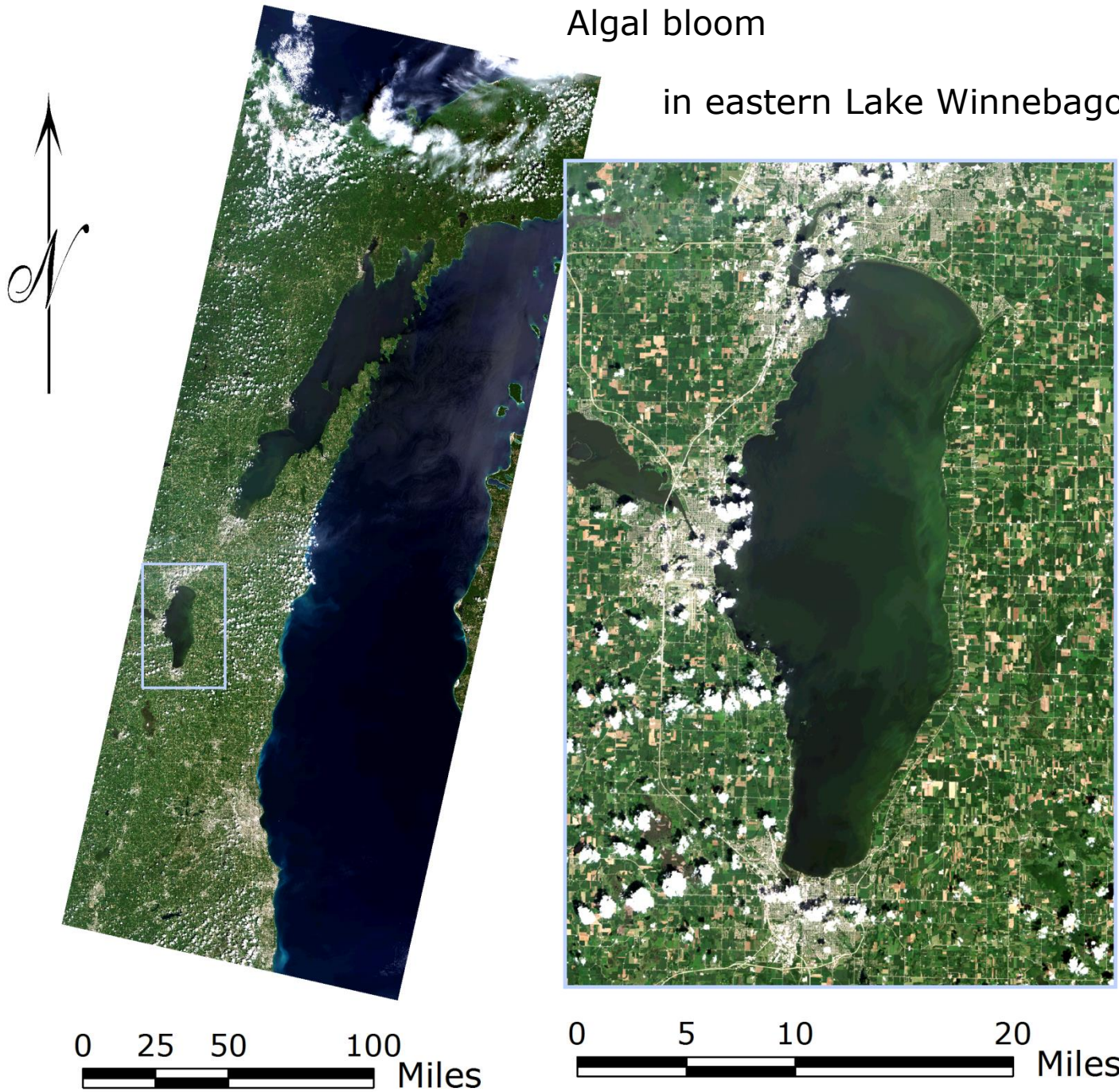
Algal bloom in eastern Lake Winnebago as seen by Landsat 8 OLI on 07/26/2016 (Source of Landsat 8 OLI data: U.S. Geological Survey).
